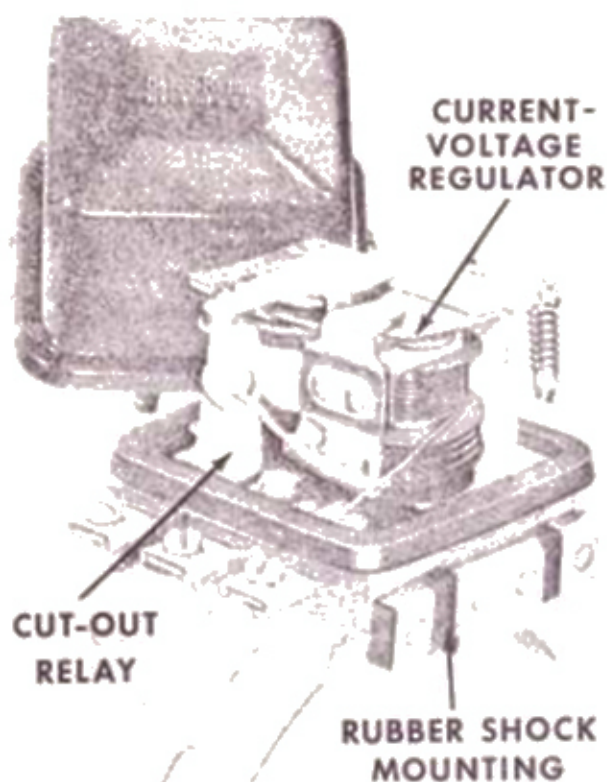
Figure 1—Delco-Remy 1118200 type combined current-voltage regulator with cover removed so units can be seen.
