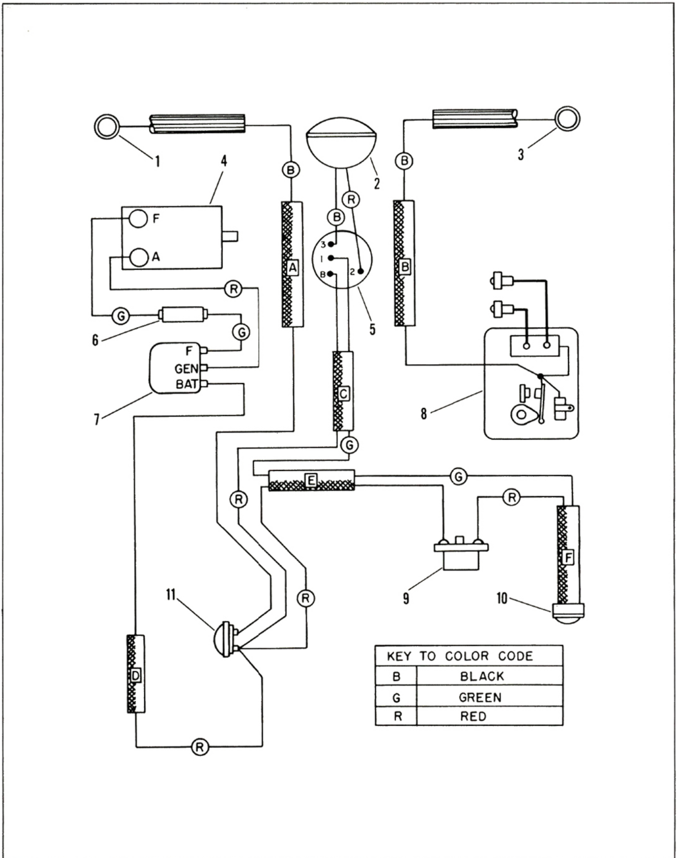
Figure 5B-7. 1959-62 Sportster CH - Wiring Diagram
